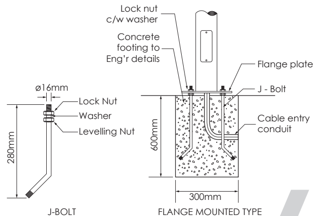
FLANGE PLATE (9mm Thickness)
