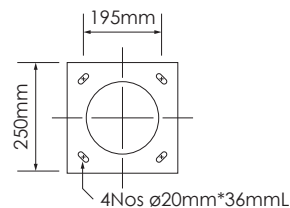
FLANGE PLATE (9mm Thickness)
