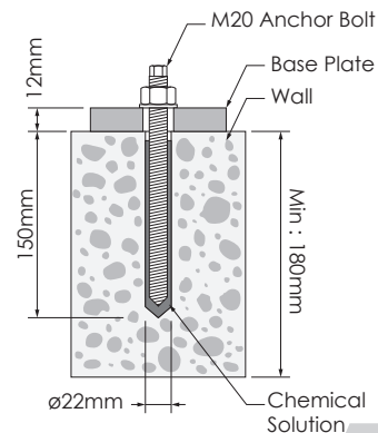
APPLICATION DIAGRAM
