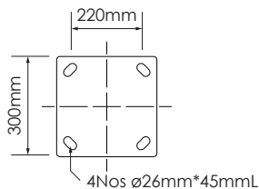
FLANGE PLATE (12mm Thickness)
