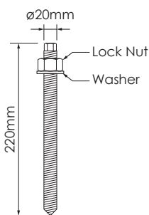
M20 CHEMICAL ANCHOR BOLT
